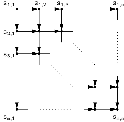
Fig. 2. Network topology of the scalable program s-m
